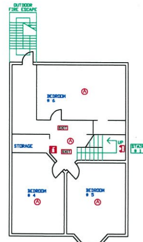
THIRD FLOOR
