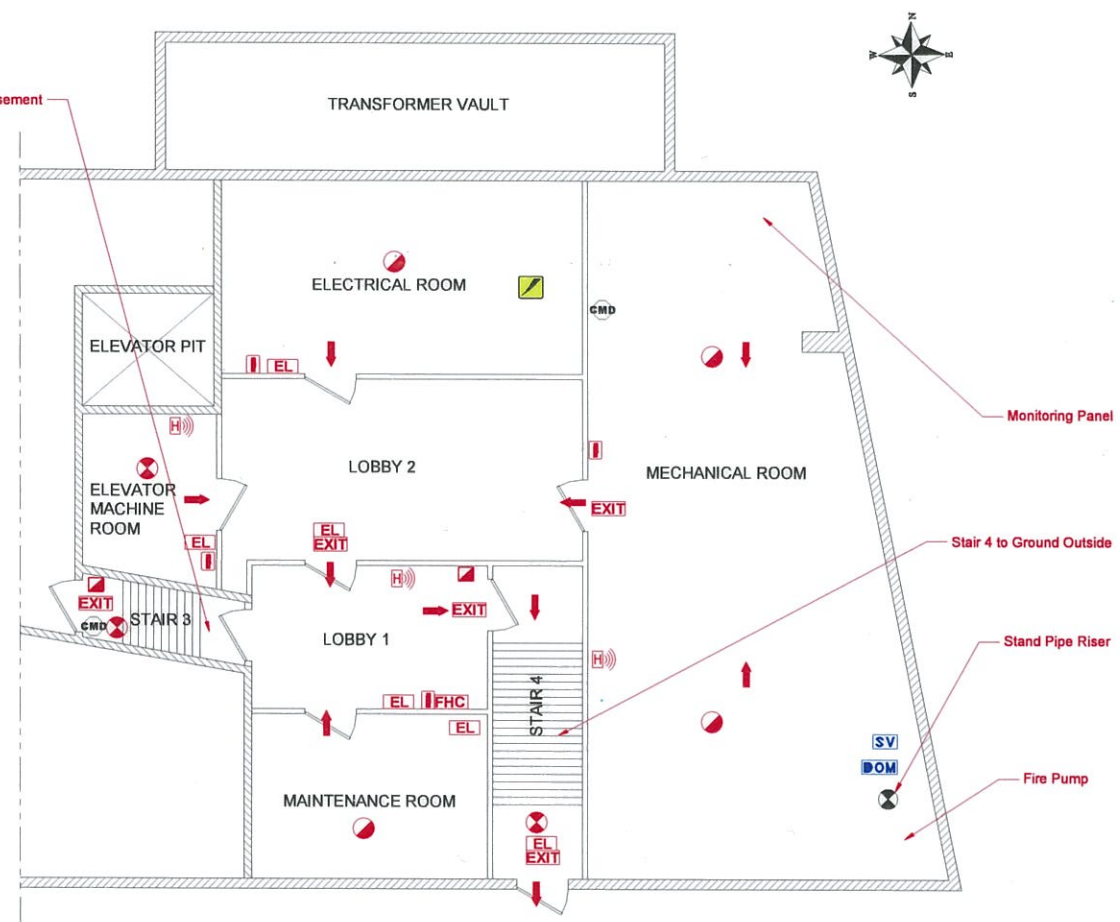
2 Basement Plan Scale: N/A
